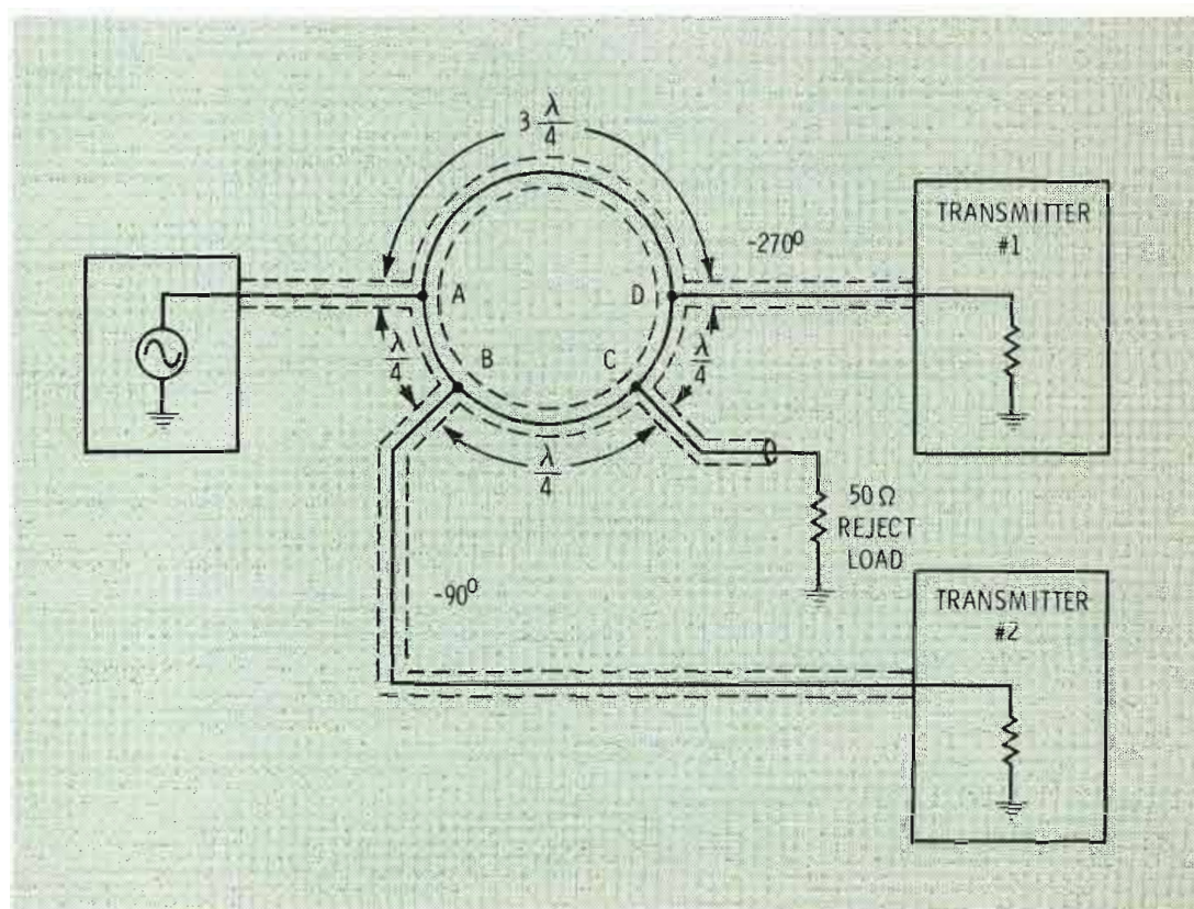
Fig. 4 The ring hybrid shown here consists of a series of quarterwave coax sections arranged in a circle.
