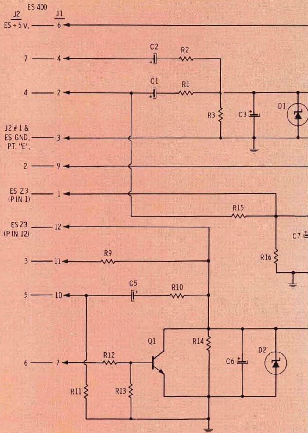
Fig. 1 Timer/recorder interface schematic.
