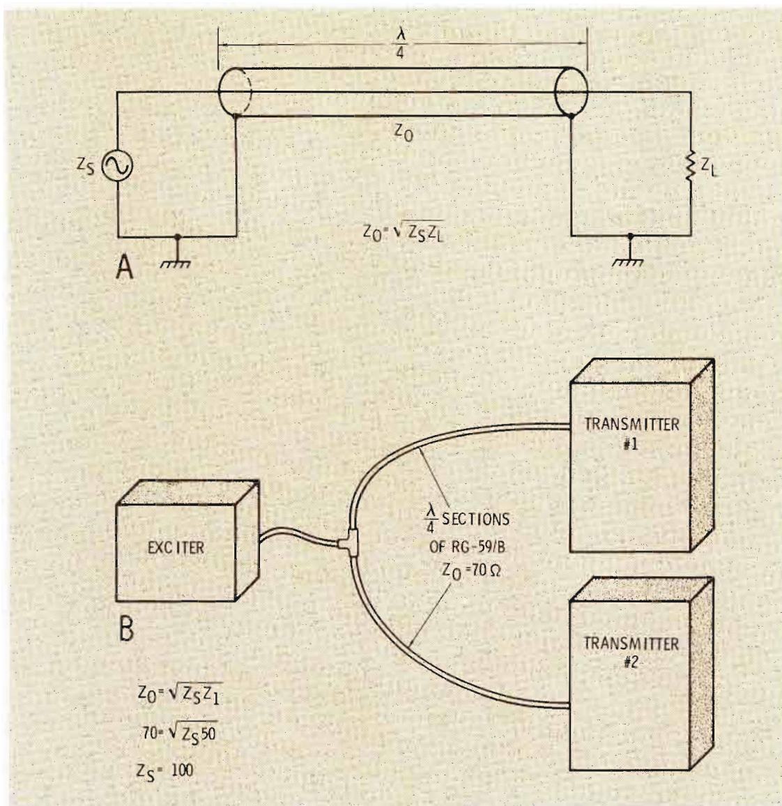
Fig. 2 At "A", unequal source and load impedance can be matched. At "B", two 100 Ohm loads are paralleled to effect an acceptable load to the exciter.
